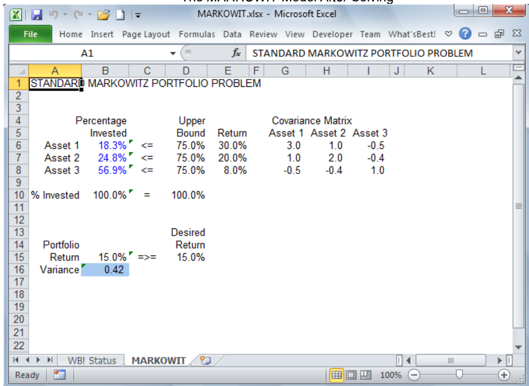
The MARKOWIT Model After Solving
