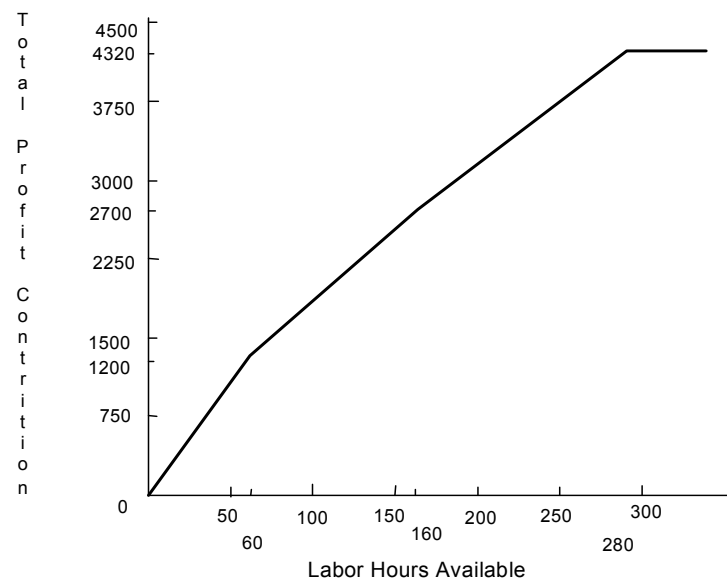
Figure 3.2 Profit vs. Labor Available
