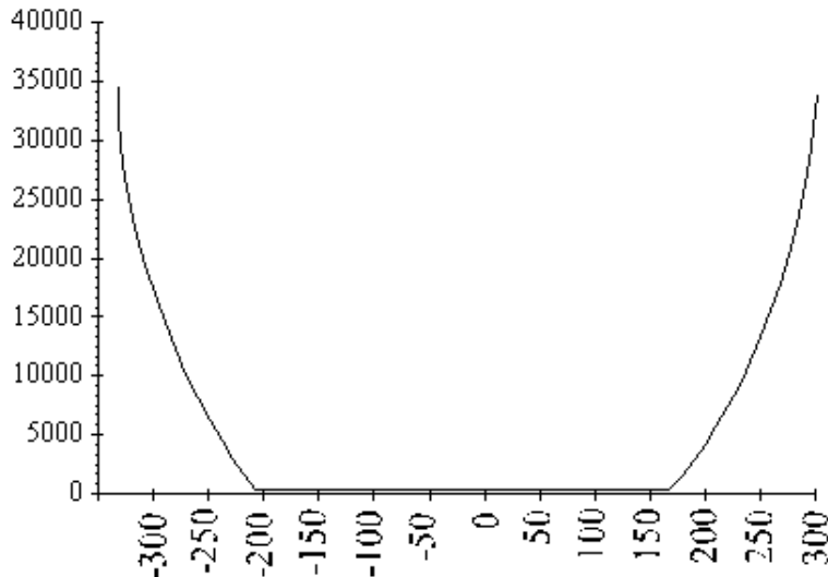
A Loosely Convex Function
